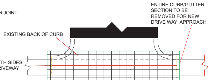
DRIVEWAY INSTALLATION AT EXISTING CURB/GUTTER
