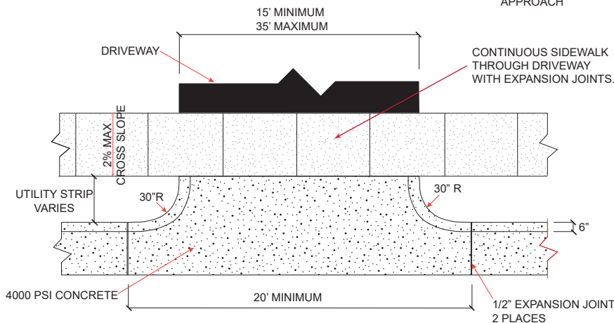
STANDARD DRIVEWAY CONSTRUCTION WITH SIDEWALK
