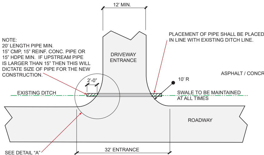
STANDARD DRIVEWAY CONSTRUCTION EXISTING DEVELOPMENT WITH NO CURB & GUTTER
