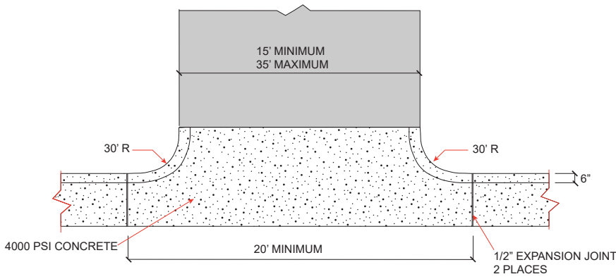
STANDARD DRIVEWAY CONSTRUCTION
